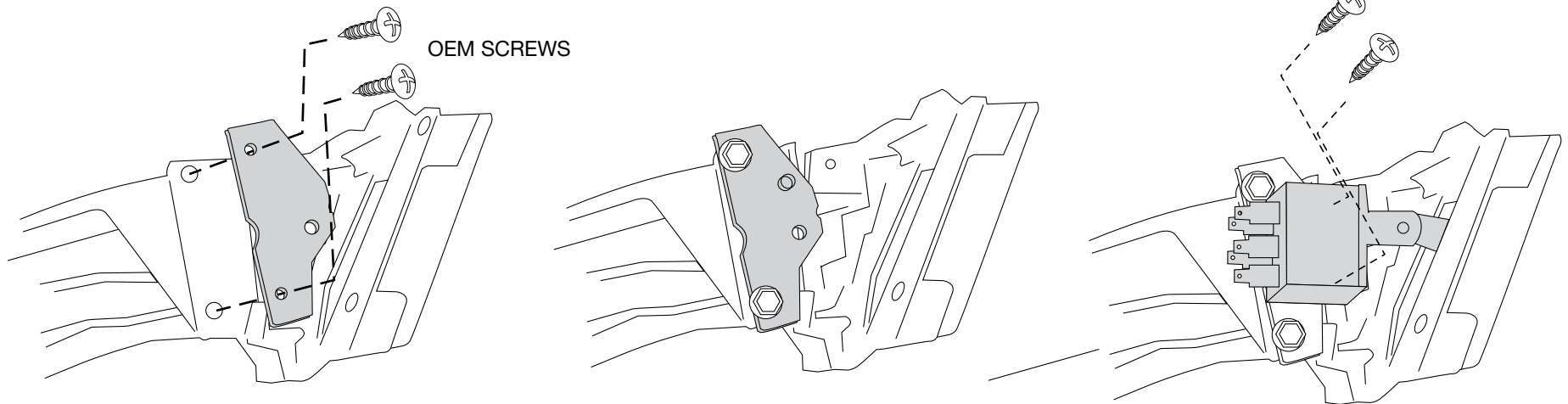
Two #8 - 20x3/8" Screws
