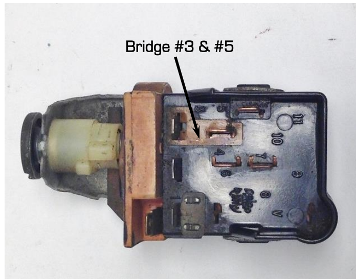
Figure 8 - Headlight Switch
