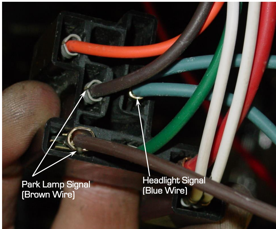
Figure 7 – Locating the Brown & Blue Wires
