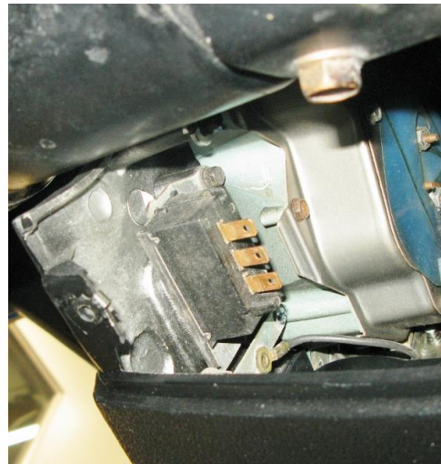
Figure 3 – Remove Stock Wiper Switch & Connector
