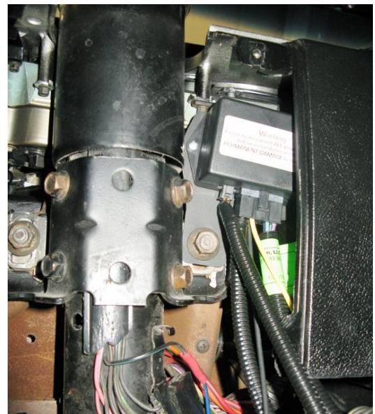
Figure 11 – Connect Wiper Switch & Harness to Module
