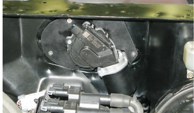
Figure 2 - Wiper Motor Orientation (P/N: 121406 Shown)
