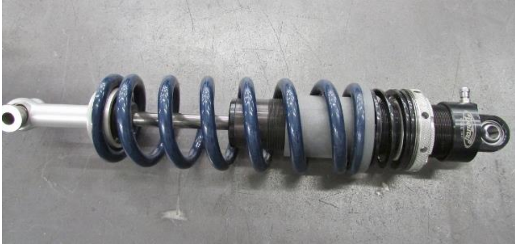
Figure 14 - Assembled Coilover Shock & Spring
