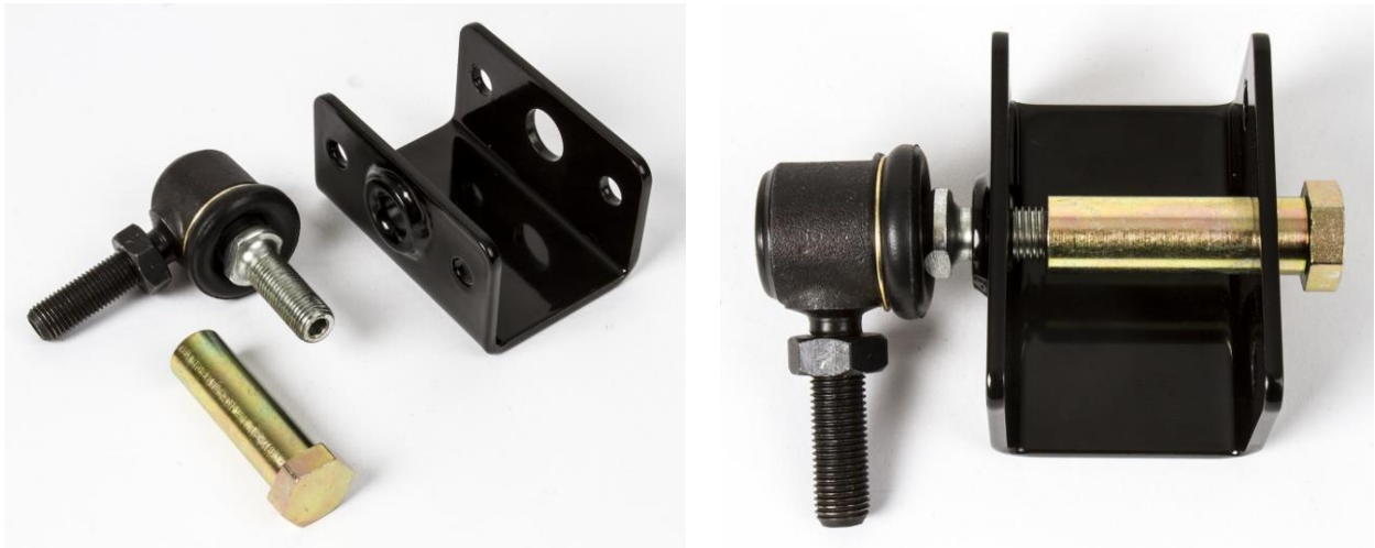
Figure 10 – ARB Mounting Bracket, Upper End Link & Frame Mount Bracket Nut
