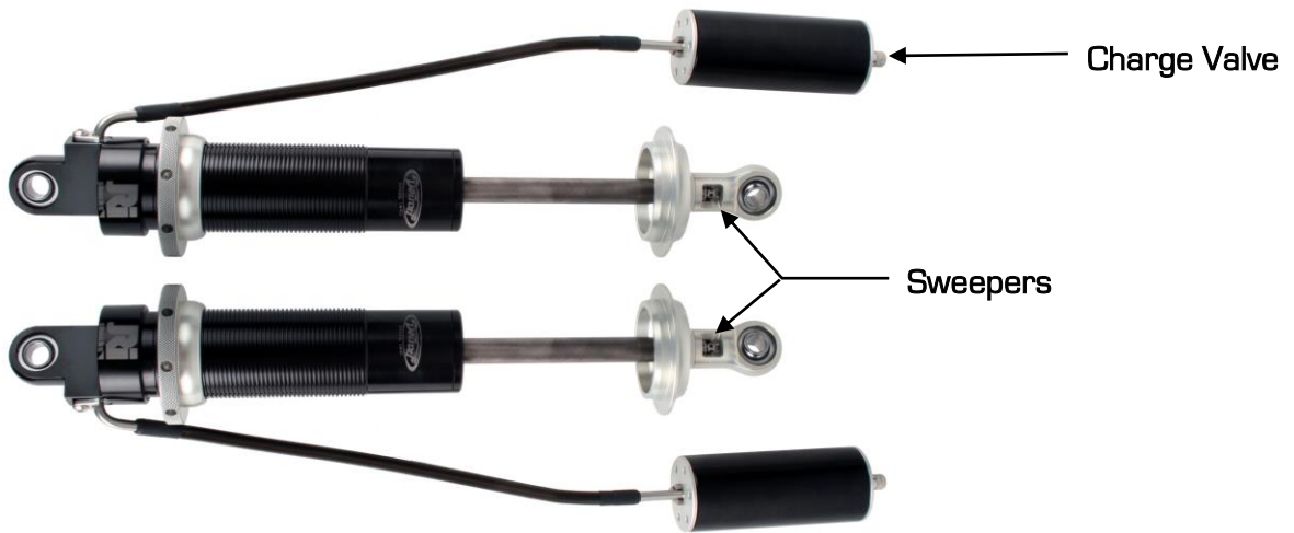
Figure 13a – Detroit Speed Double Adjustable Shock w/Remote Canister
