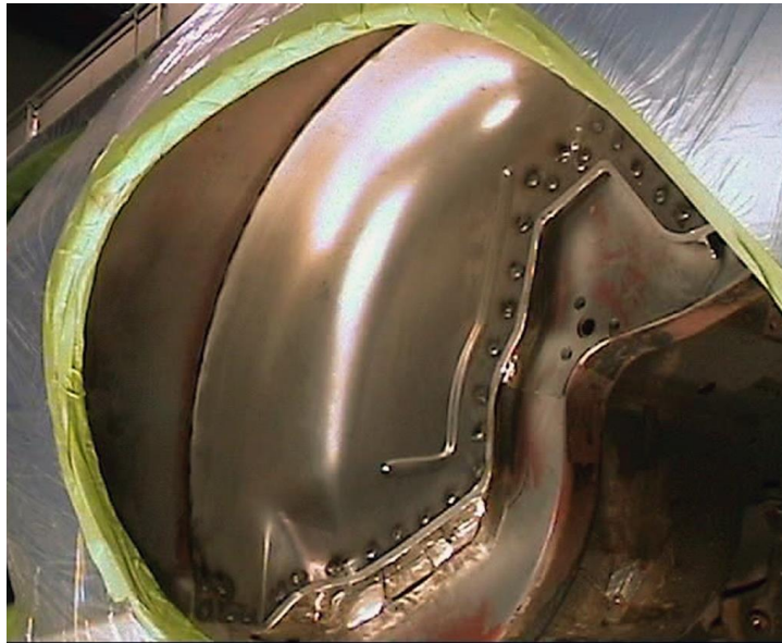
Figure 18 – Weld Mini-Tub to Side Flanges
