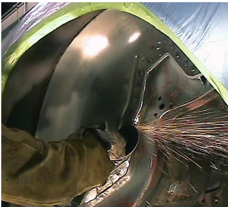
Figure 19 – Smooth Spot Welds
