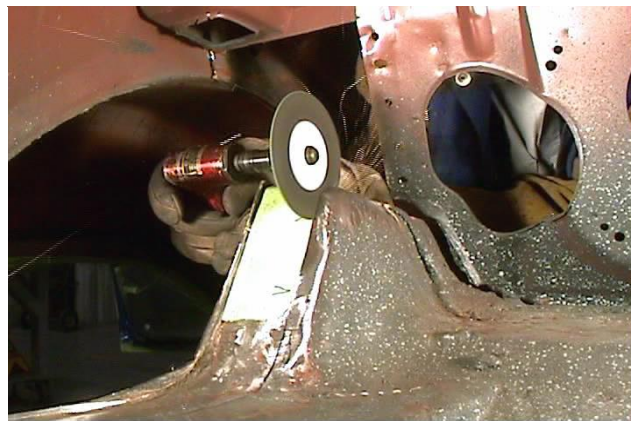
Figures 8 & 9 - Metal Removal for Clearance of DSE Deep Tubs
