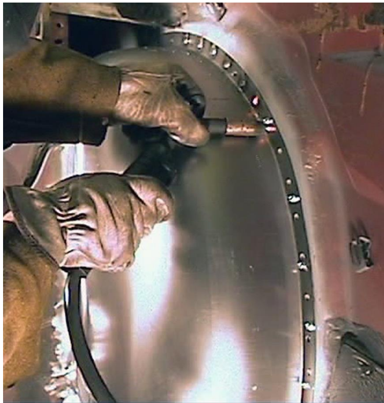
Figure 17 – Plug Weld
