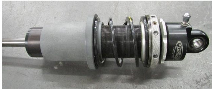
Figure 2 - Install Spring Divider
