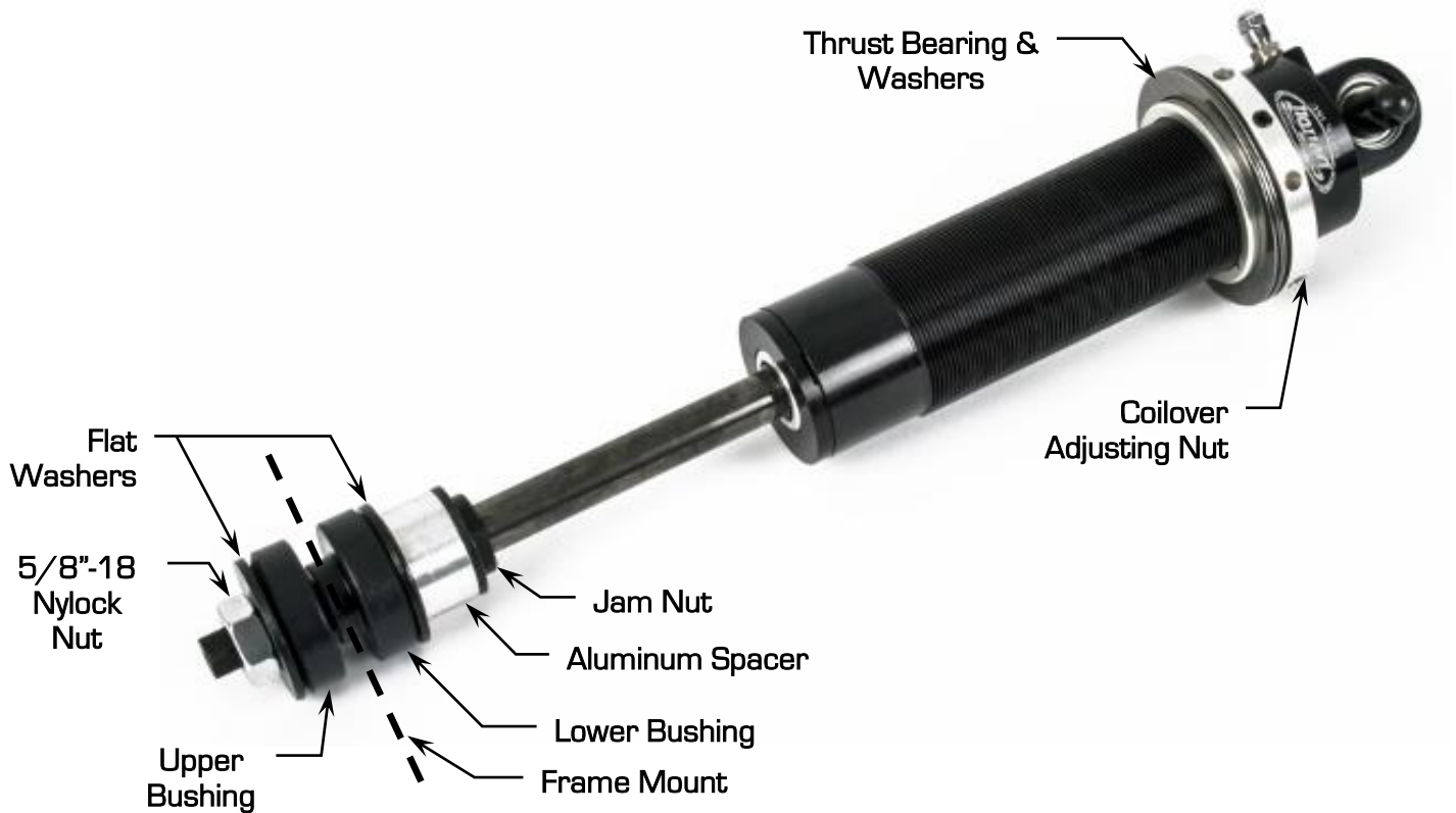
Figure 1 - Shock Assembly
