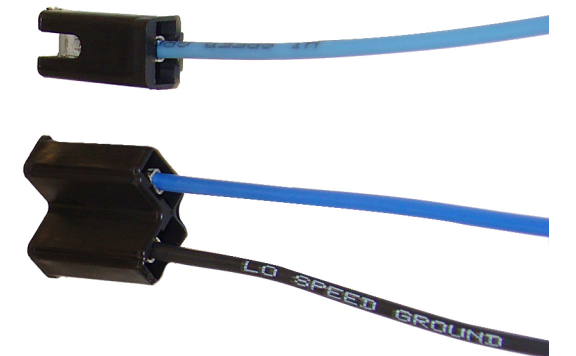
FIGURE #5 1963 - 66 SWITCH CONFIGURATION
